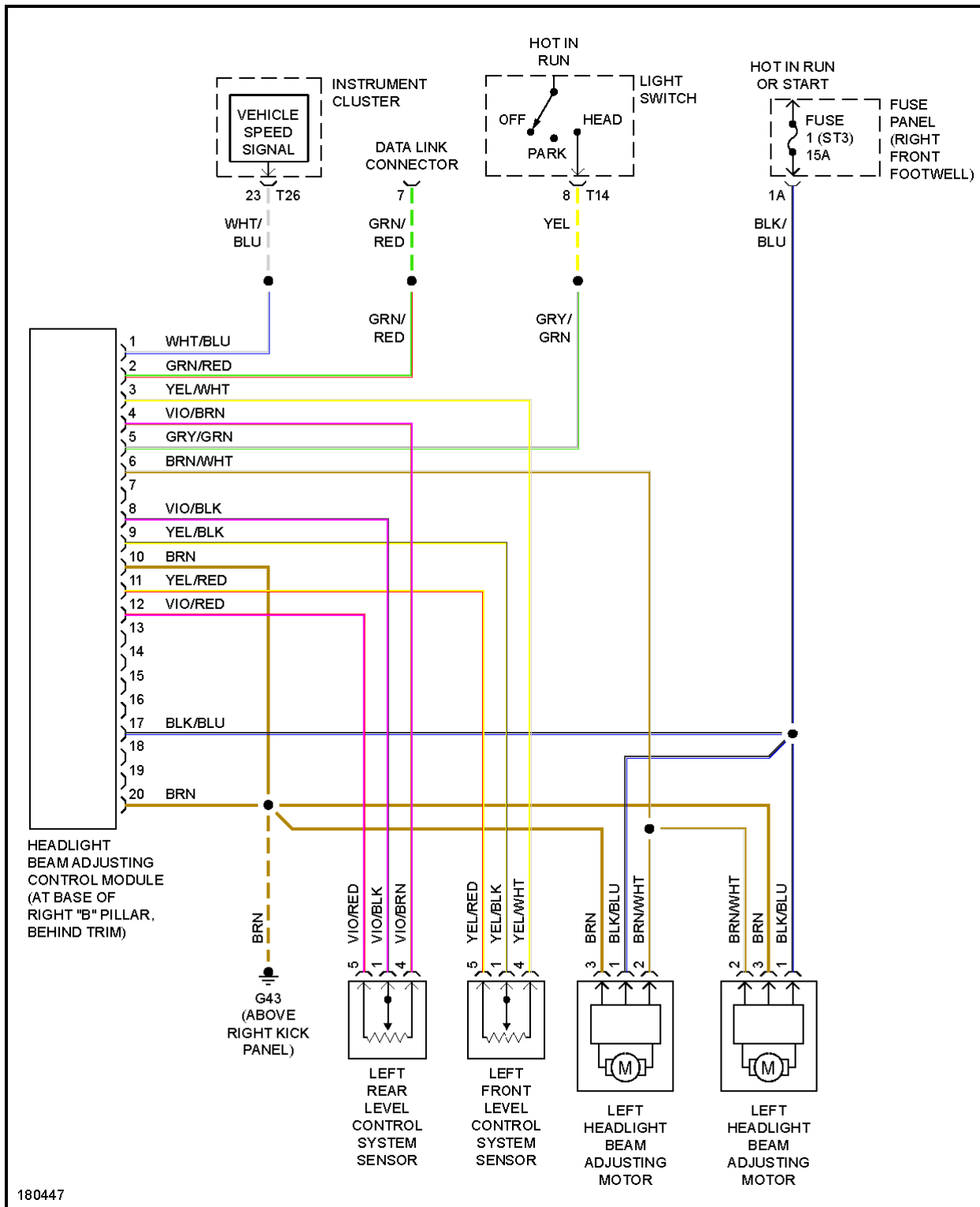
Fig. 27: Headlamp Beam Adjustment Circuit
